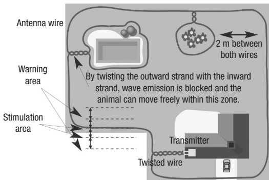
Diagram 4 – Sample installation
