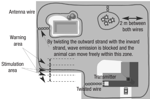
Diagram 3 – Sample installation
