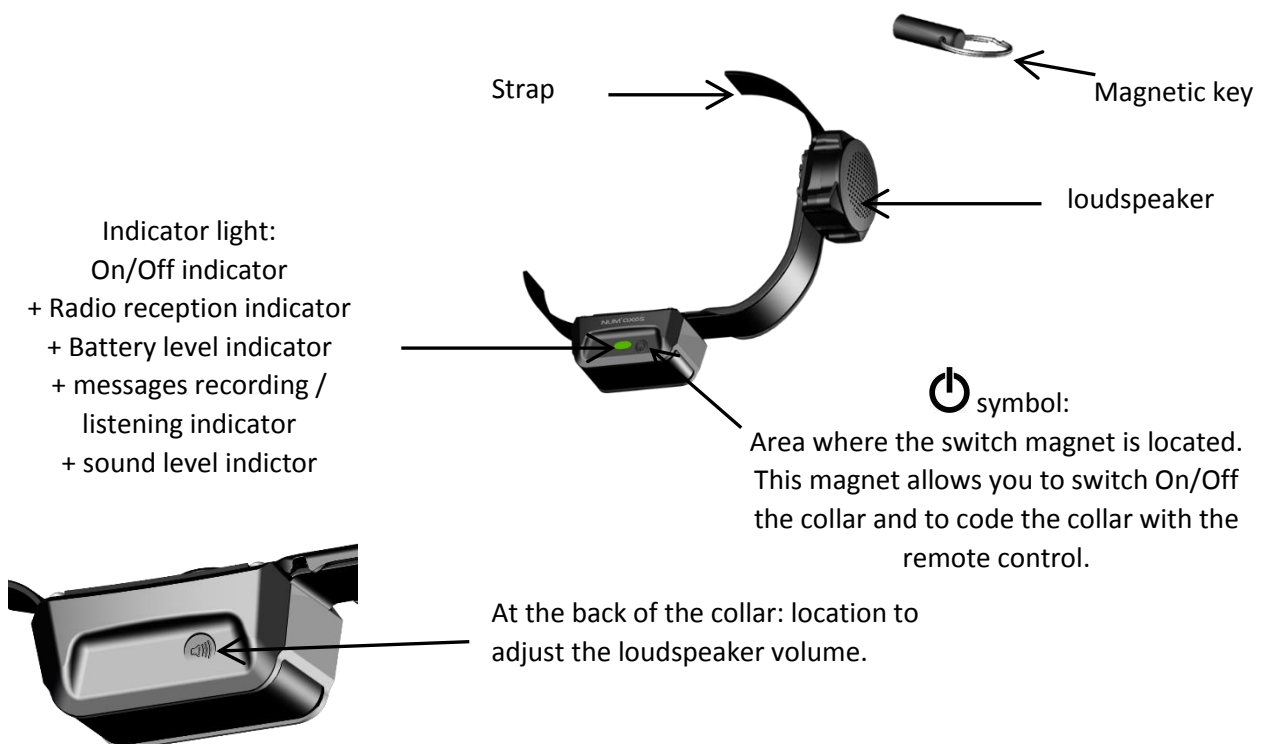
Diagram 1 Receiver collar
