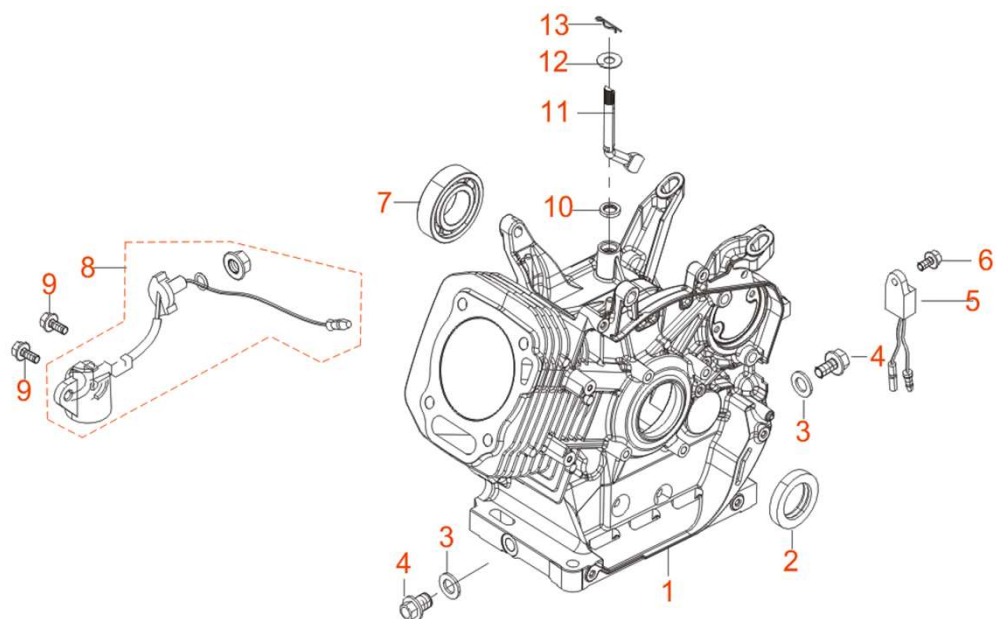
FIG.2 CRANKCASE (E02)
