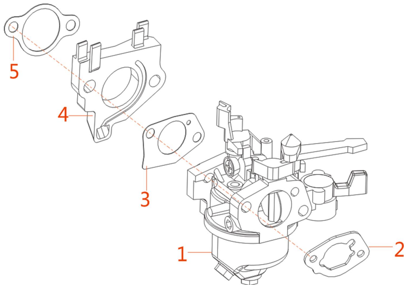
FIG.8 CARBURETOR ASSY (E8)
