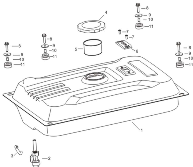
FIG.11 TANK ASSY, FUEL (F11)
