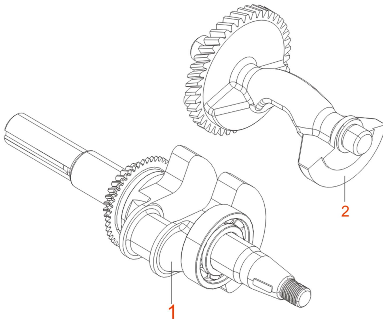
FIG.4 ROD,CRANKSHAFT CONNETING (E04)
