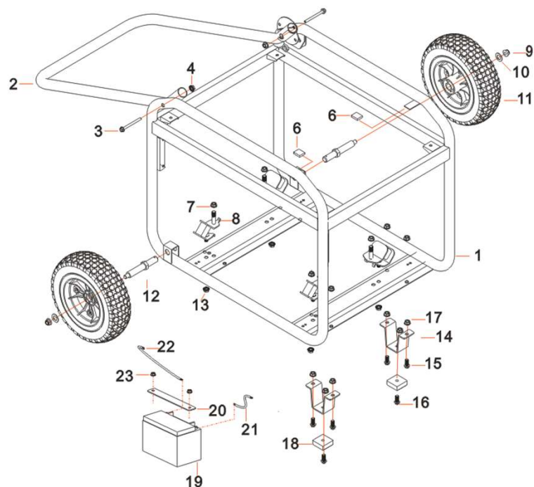
FIG.14 FRAME, ENGINE (E14)
