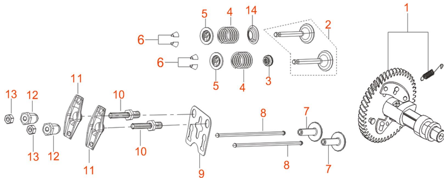
FIG.6 TRAIN,VALVE / CAMSHAFT SUBASSEMBLY (E06)
